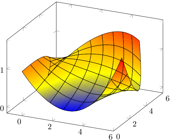
Mesh on top of patches (i): obscured
