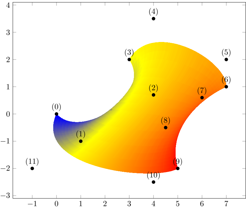
A Coons Patch
