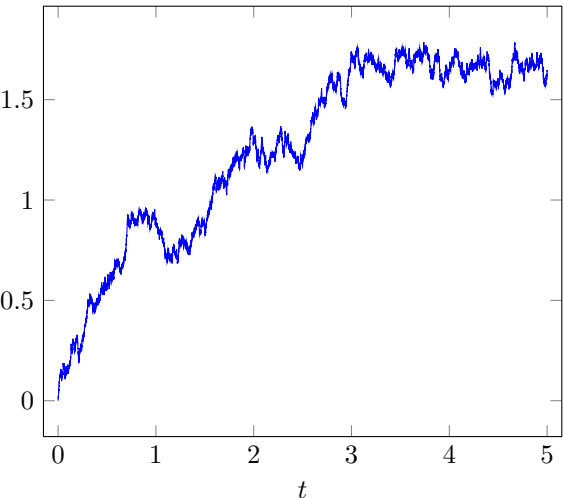
Ornstein-Uhlenbeck sample (13000 time steps)
